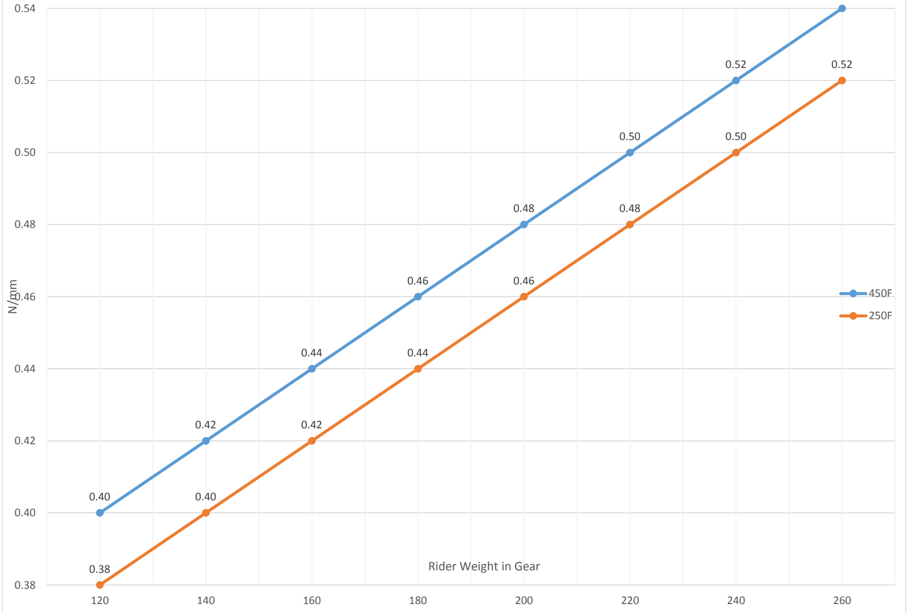
14-16YZF Fork Spring Rate
